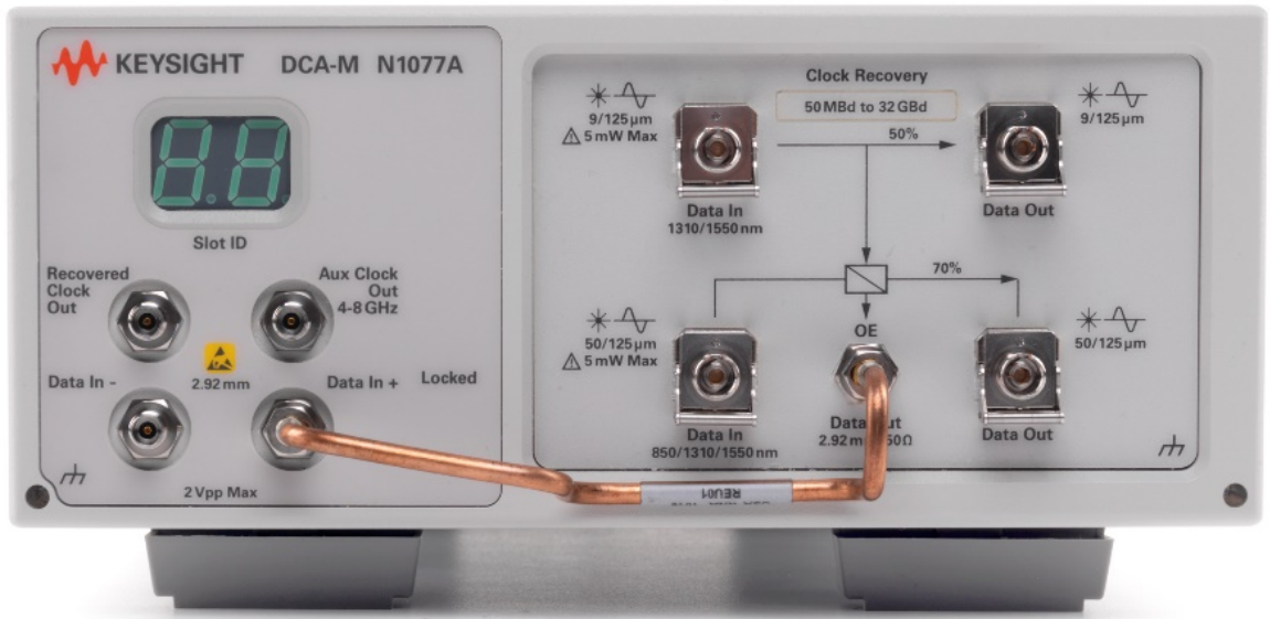
Figure 26: N1077A Single- & multimode optical/electrical clock recovery with options 232 and SMS
